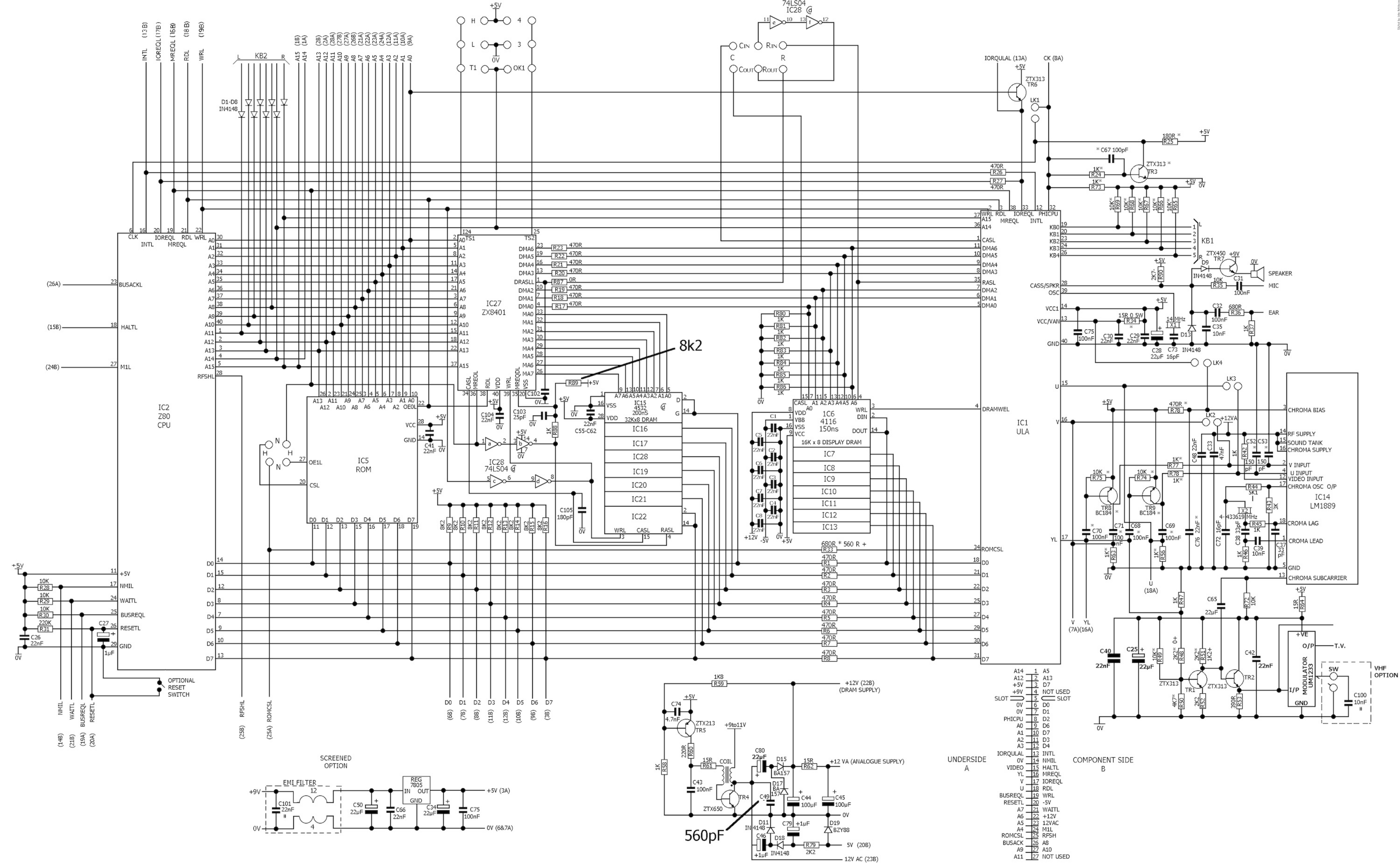
ZX SPECTRUM (ISSUE 6A) CIRCUIT DIAGRAM FIGURE 6
